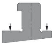
AS I schultertragend
